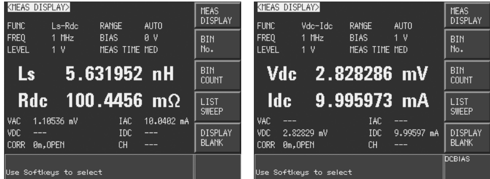
Figure 14. DCR, DCV and DCI measurements
