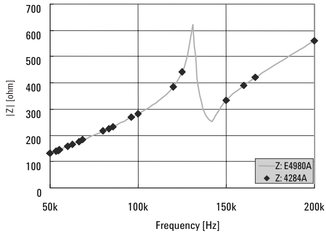
Figure 12. Increased frequency resolution enhances test accuracy
